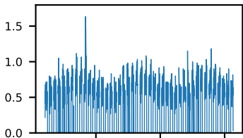
60-s bins
