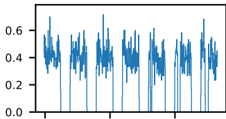
60-s bins
