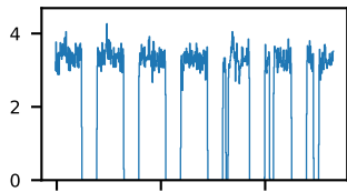
60-s bins
