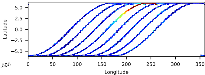
80202006004: 3 to 10 keV
