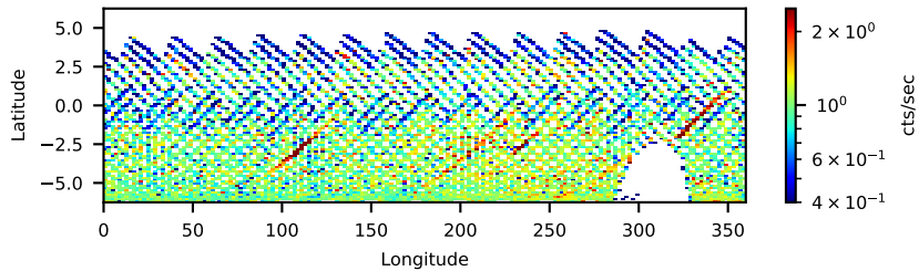
70901001002: 3 to 120 keV
