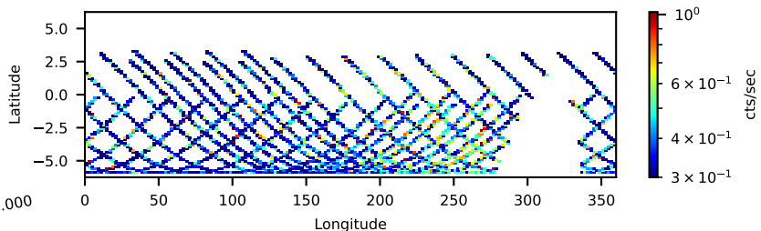
70660003004: 30 to 120 keV
