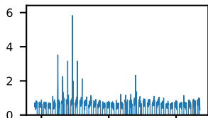
60-s bins
