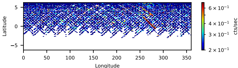
61101003002: 3 to 10 keV
