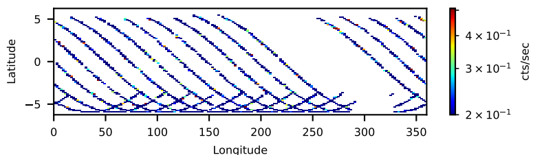
61064003002: 3 to 10 keV
