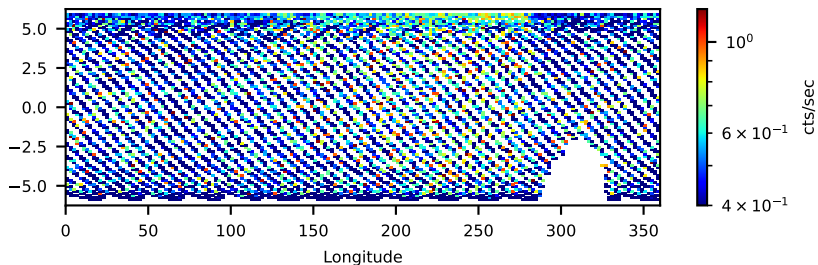
61002011002: 3 to 10 keV
