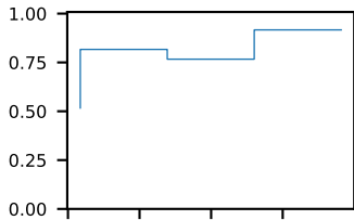
60-s bins
