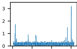
60-s bins
