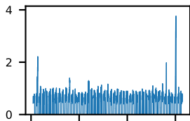
60-s bins
