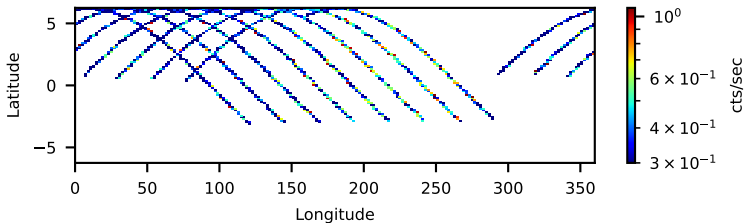
60802036004: 30 to 120 keV
