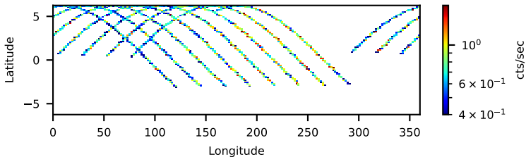
60802036004: 3 to 120 keV
