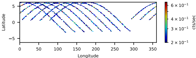
60802036004: 3 to 10 keV
