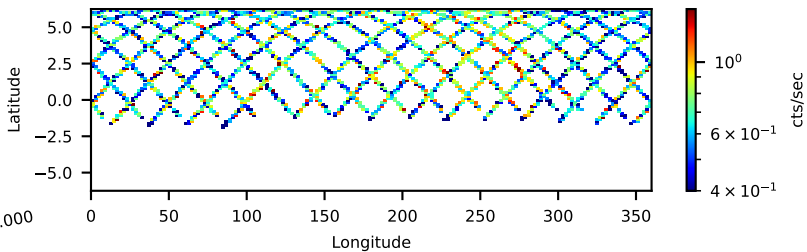
60802036002: 3 to 10 keV
