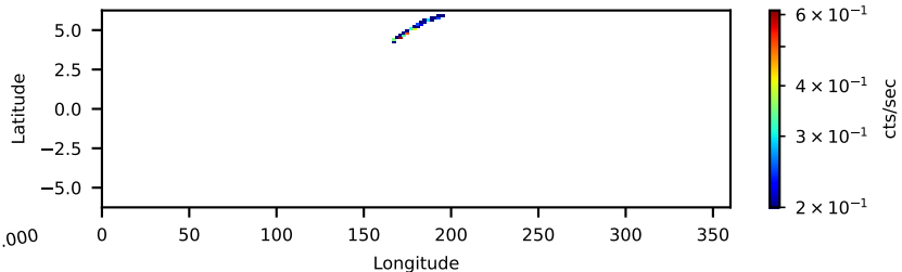
60802036001: 30 to 120 keV
