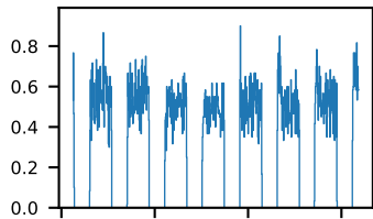
60-s bins
