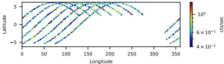
60802002020: 3 to 120 keV
