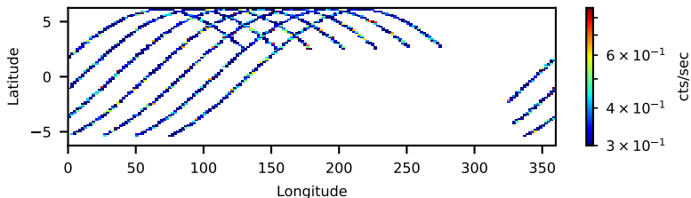
60802002020: 30 to 120 keV
