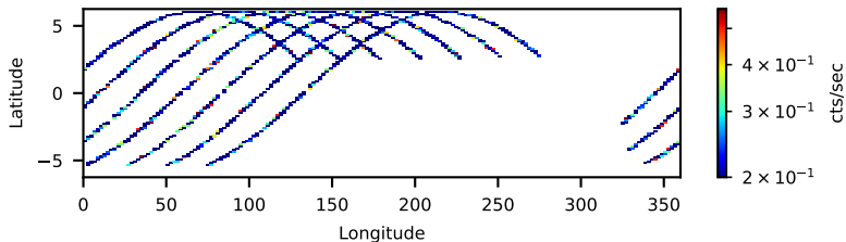
60802002020: 3 to 10 keV
