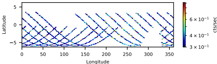
60801018002: 30 to 120 keV
