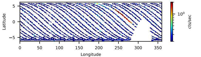
60763001002: 3 to 10 keV
