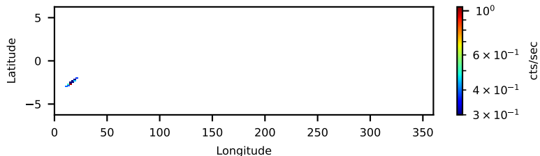
60702018007: 30 to 120 keV
