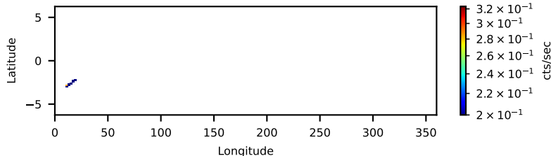
60702018007: 3 to 10 keV
