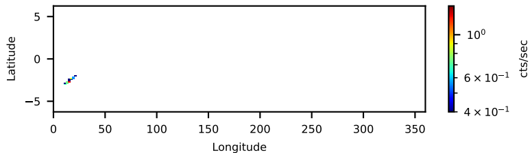
60702018007: 3 to 120 keV
