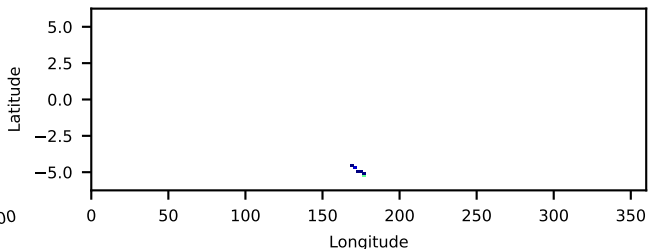
60701063003: 30 to 120 keV
