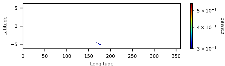
60701063003: 30 to 120 keV
