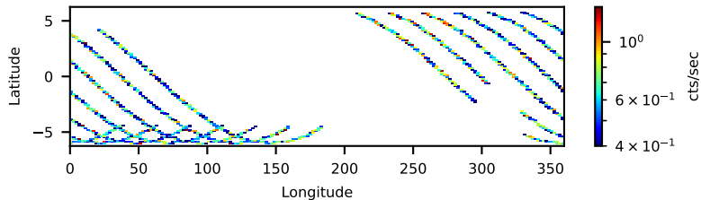
60701019002: 3 to 120 keV
