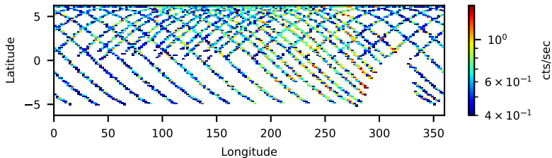
60666015002: 3 to 120 keV
