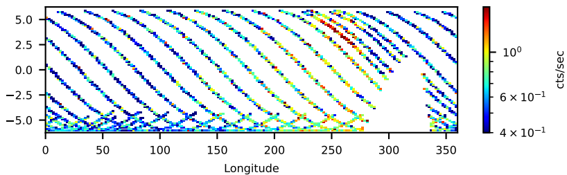
60502006004: 3 to 10 keV
