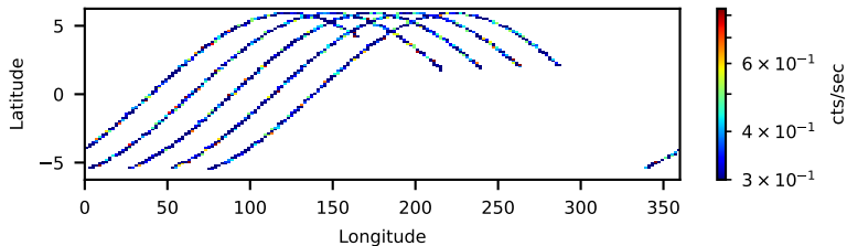
60464183002: 30 to 120 keV
