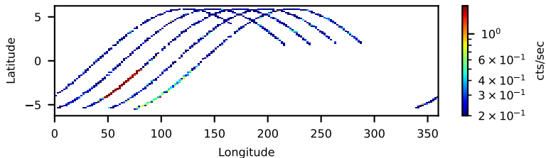
60464183002: 3 to 10 keV
