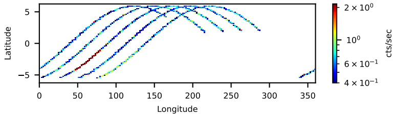
60464183002: 3 to 120 keV
