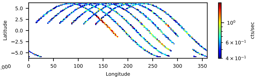
60464165002: 3 to 10 keV
