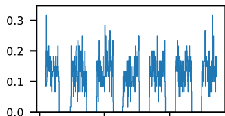
60-s bins
