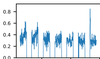
60-s bins
