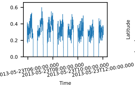
60-s bins
