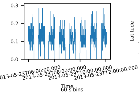
60-s bins
