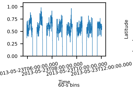
60-s bins
