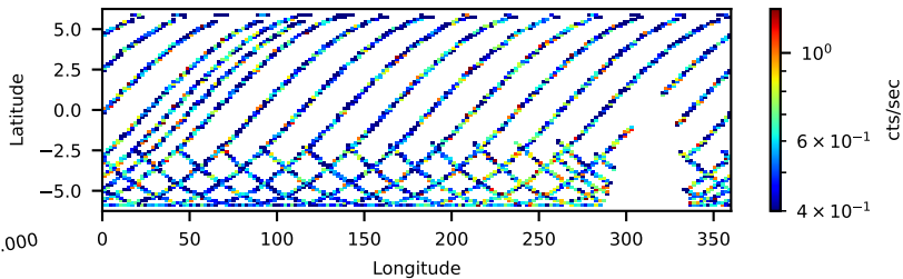
60023006005: 3 to 10 keV
