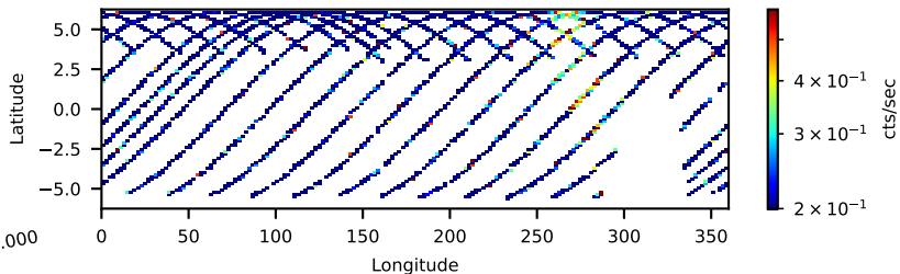
60022015003: 30 to 120 keV
