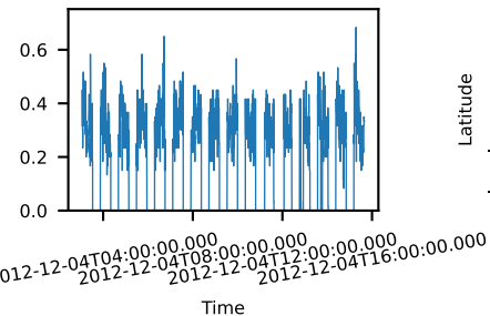
60-s bins
