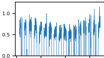
60-s bins
