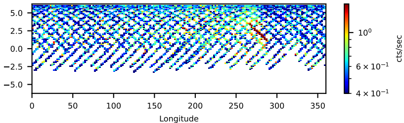
60001158002: 3 to 10 keV
