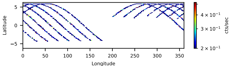
60001144002: 3 to 10 keV
