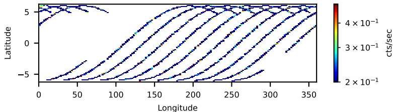
50910009002: 3 to 10 keV
