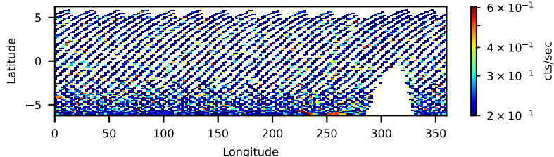
50910005002: 3 to 10 keV
