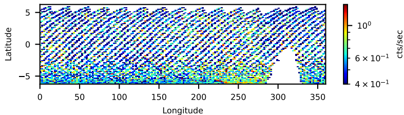
50910005002: 3 to 120 keV
