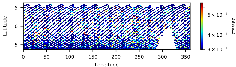
50910005002: 30 to 120 keV
