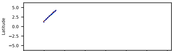
50901001001: 3 to 10 keV
