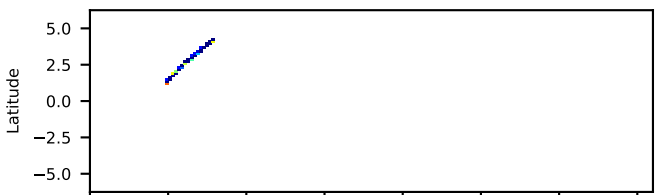
50901001001: 30 to 120 keV
