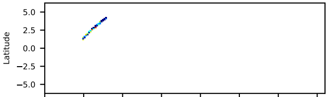
50901001001: 3 to 120 keV
