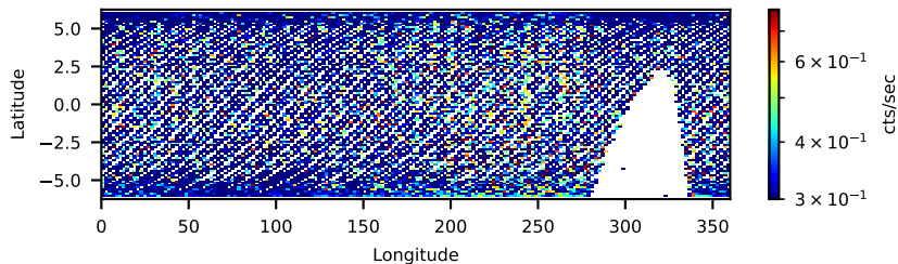
50401001002: 30 to 120 keV
