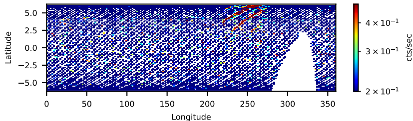
50401001002: 3 to 10 keV
