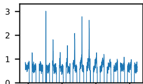
60-s bins
