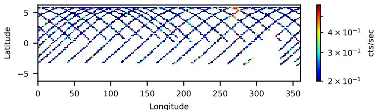
50312002002: 3 to 10 keV
