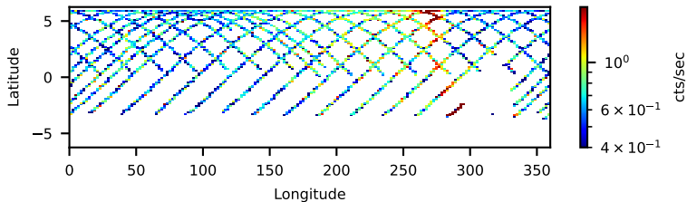
50312002002: 3 to 120 keV
