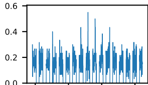
60-s bins
