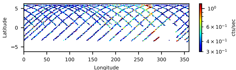
50312002002: 30 to 120 keV
