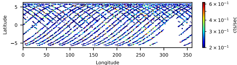
50311003004: 3 to 10 keV
