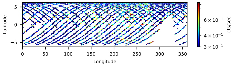
50311003004: 30 to 120 keV
