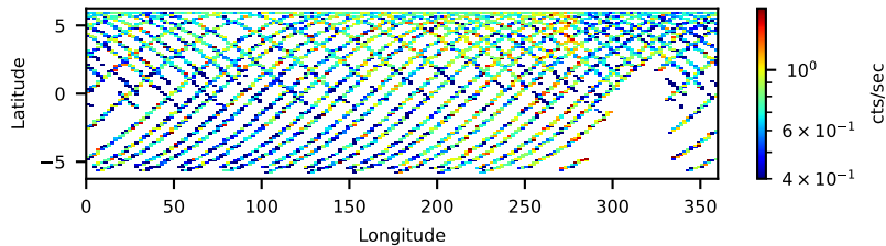
50311003004: 3 to 120 keV
