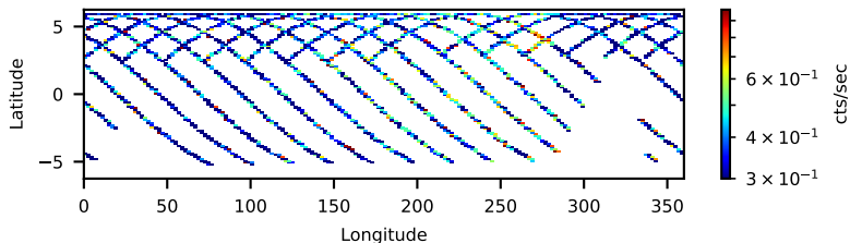
50302001002: 30 to 120 keV
