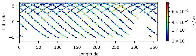
50302001002: 3 to 10 keV
