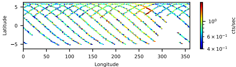
50302001002: 3 to 120 keV
