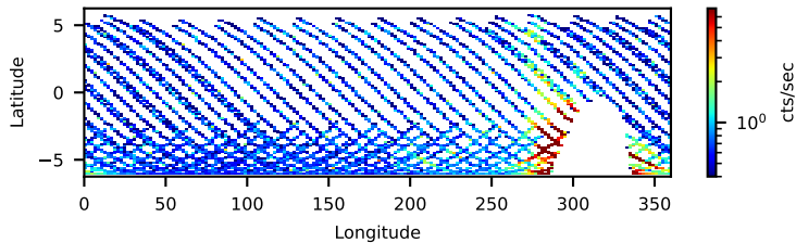
50111001002: 3 to 120 keV
