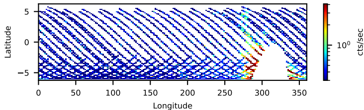
50111001002: 30 to 120 keV
