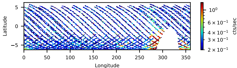
50111001002: 3 to 10 keV
