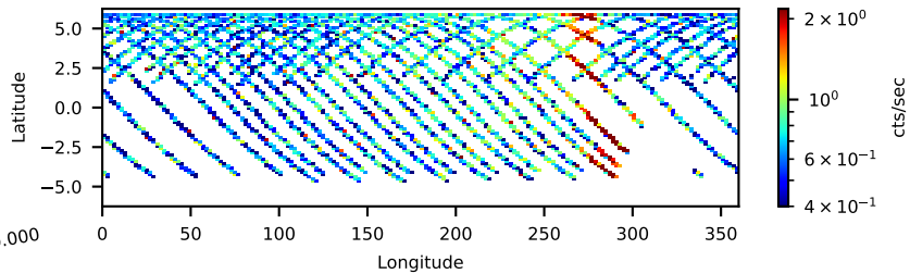
50110001004: 3 to 10 keV
