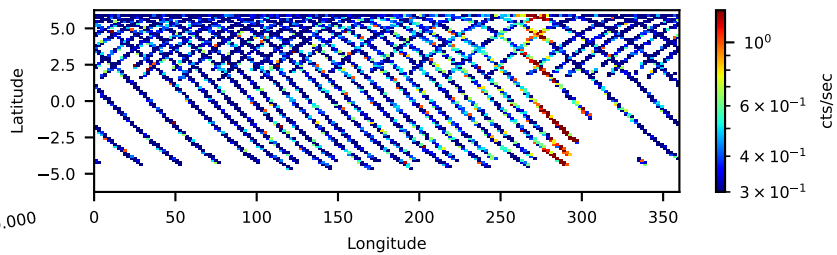
50110001004: 30 to 120 keV
