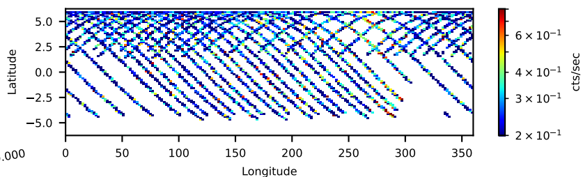
50110001004: 3 to 10 keV
