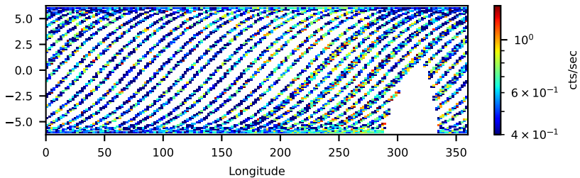
50026003002: 3 to 10 keV
