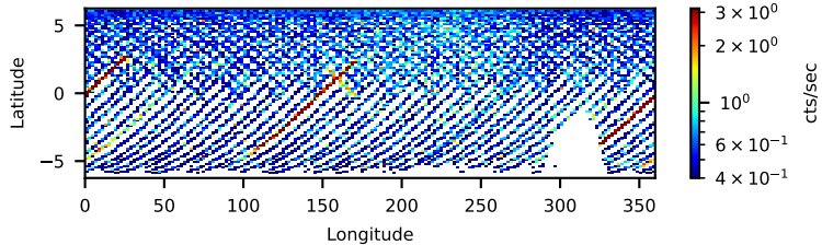
40901005002: 3 to 120 keV
