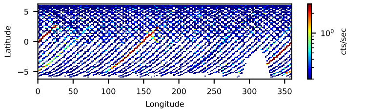
40901005002: 3 to 10 keV
