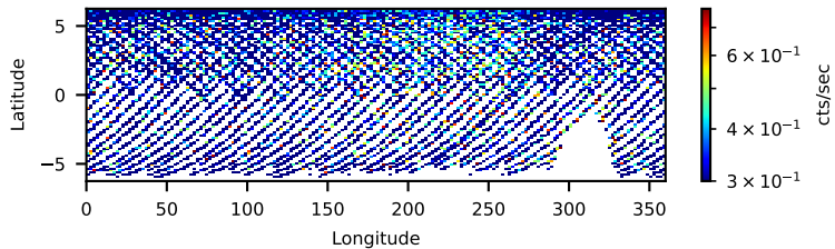
40901005002: 30 to 120 keV
