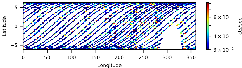
40801006002: 30 to 120 keV
