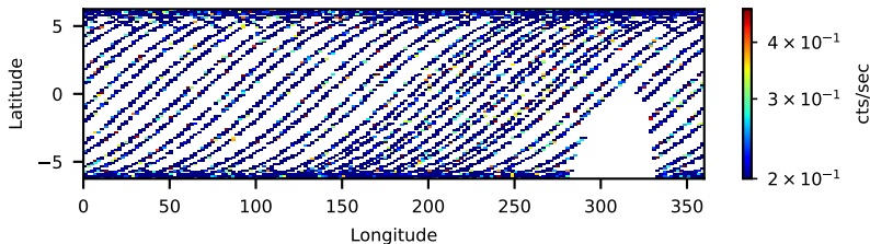
40801006002: 3 to 10 keV
