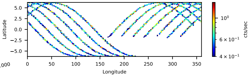
31002003008: 3 to 10 keV
