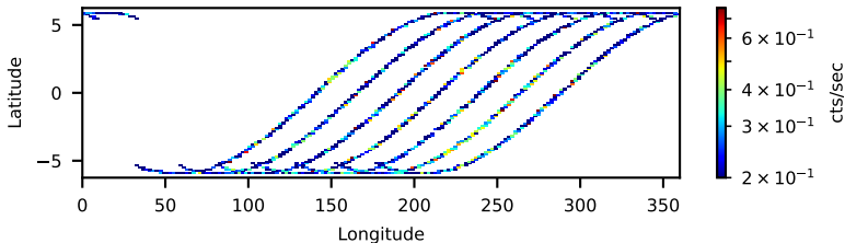
31002003002: 3 to 10 keV
