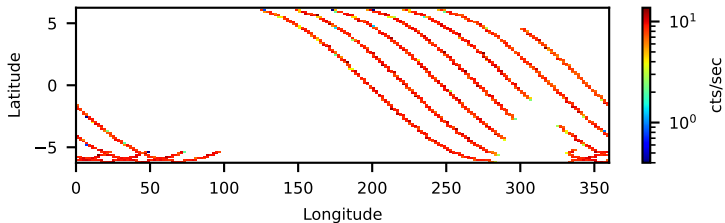
30902036002: 3 to 120 keV
