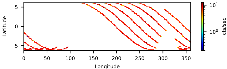
30902036002: 3 to 10 keV
