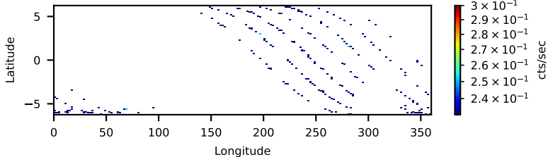
30902036002: 30 to 120 keV
